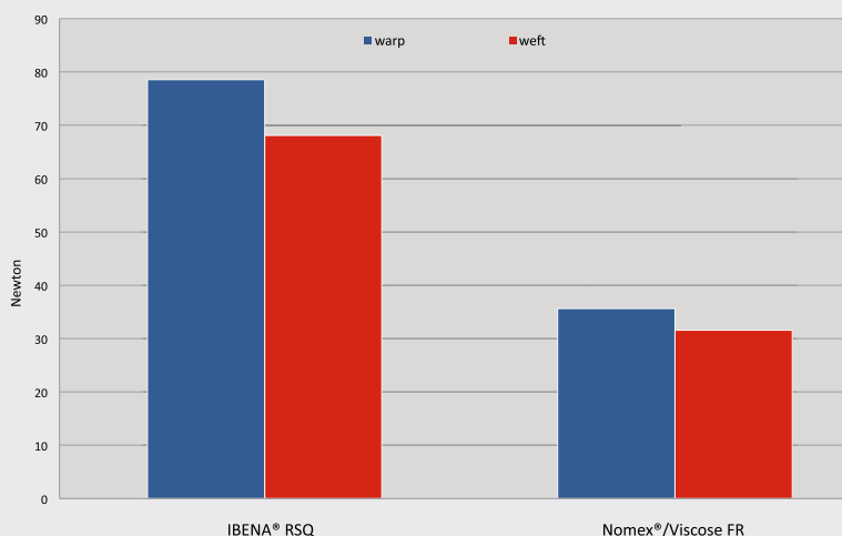
Average tear strength in accordance to DIN EN ISO 13937-2
