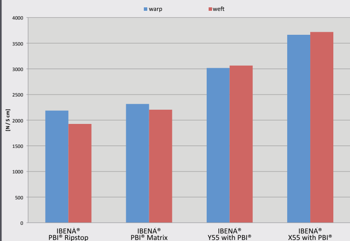
Average tensile strength in accordance to DIN EN ISO 13934-1
