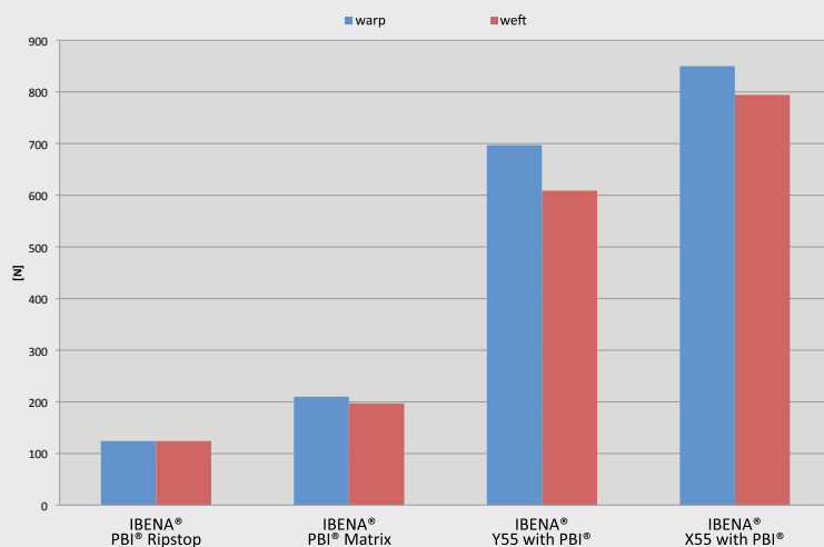
Average tear strength in accordance to DIN EN ISO 13937-2, Appendix D
