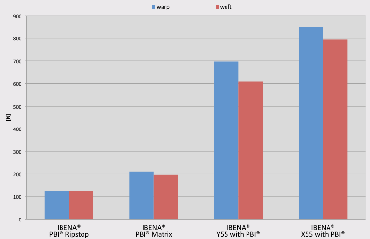
Average tear strength in accordance to DIN EN ISO 13937-2, Appendix D
